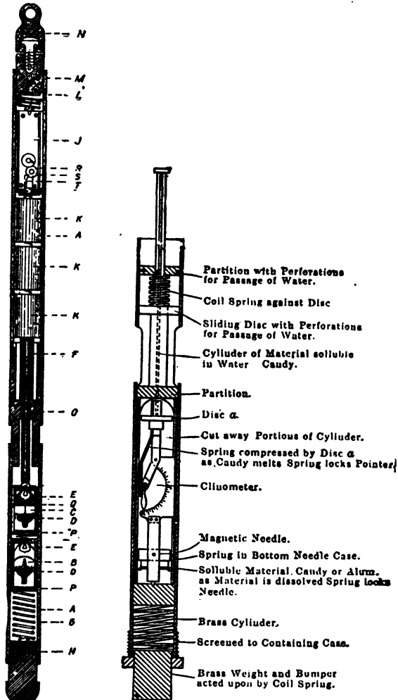
Fig. 62. Section of Surveying Instrument for Diamond Drill.
